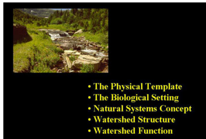
Figure 2. Five main elements of watershed ecology
